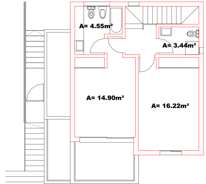
3rd Floor Area = 60.62m 2
